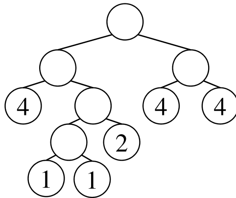
Figure I.1. A balanced tree
