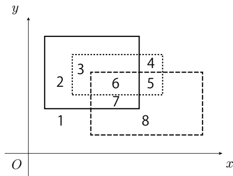
Figure C.1. Three rectangles partition the plane into eight regions. This corresponds to the first dataset of the sample input. The x - and y -axes are shown for illustration purposes only, and therefore they do not partition the plane.
