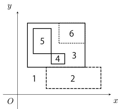
Figure C.2. Rectangles overlapping in more complex ways. This corresponds to the second dataset.
